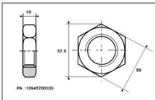
Lock-nut
