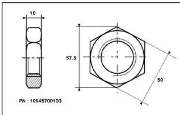
Lock-nut
