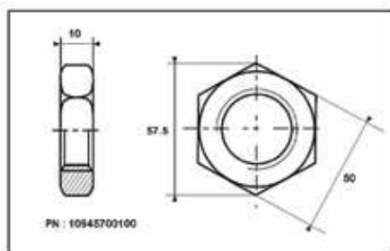
Lock-nut
