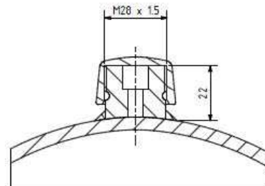
Gas Valve
